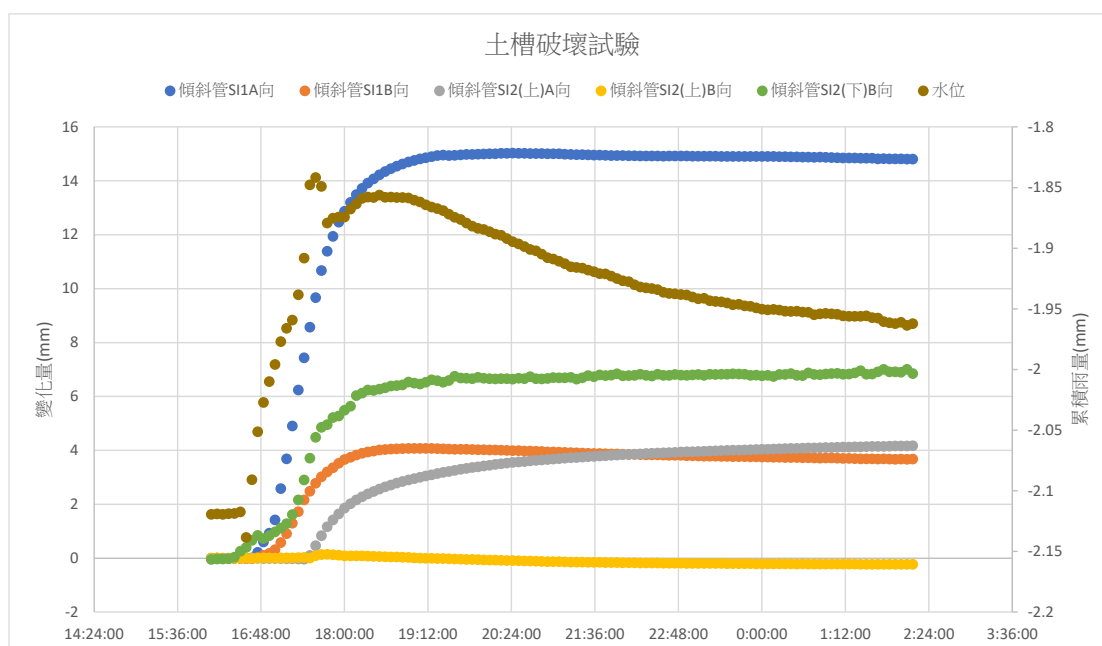
(b) 累積降雨與地層變位關係
